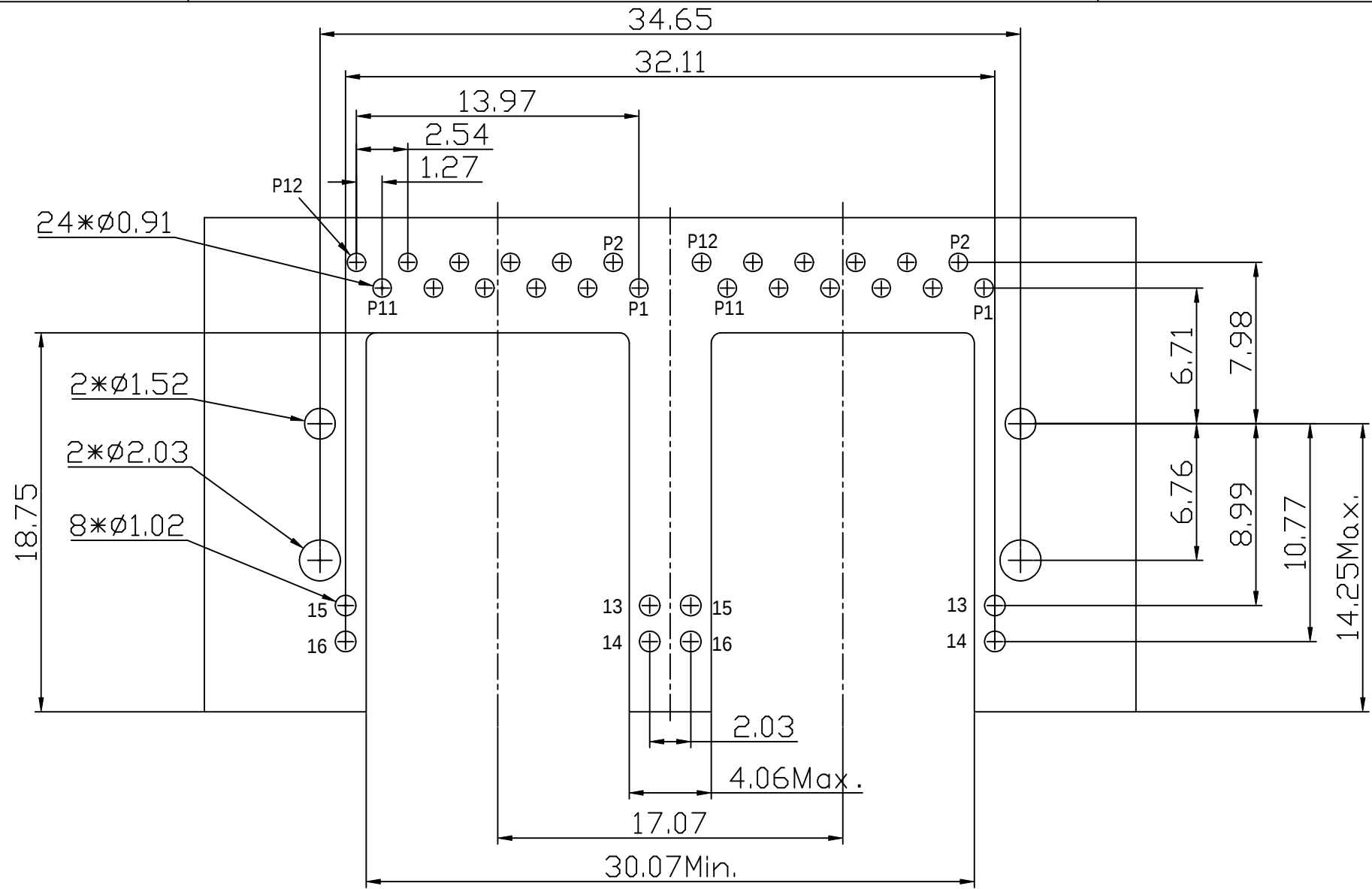
Recommended PCB Layout (Tol: ±0.05, T=1.60±0.15mm)
