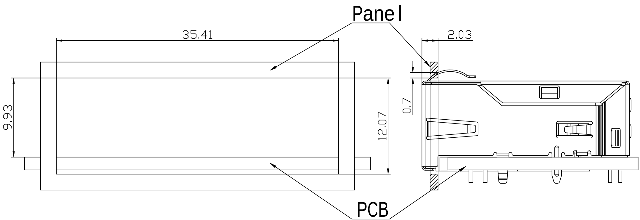
Recommended Panel Layout
